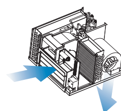
Free Cooling
