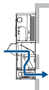
Free Cooling
